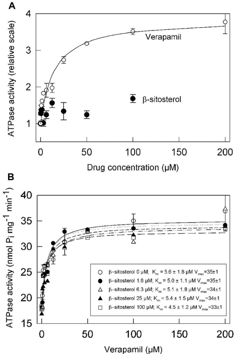
Fig. 4. Effect of sitosterol on ATPase activity. (Panel A) Relative ATPase activity in membranes isolated from P-gp-transfected Sf9 cells was measured for verapamil (○) and β-sitosterol (●) at various concentrations. The verapamil curve has been fitted to the Michaelis–Menten equation: V = V_0 + (V_{max} - V_0) S / (S + K_m) . (Panel B) Kinetics of modulation of the verapamil-stimulated P-gp ATPase activity by sitosterol was determined at 0 μM (○), 1.6 μM (●), 6.3 μM (△), 25 μM (▲) and 100 μM (□) β-sitosterol. The curves have been fitted to the Michaelis–Menten equation, and the kinetic parameters obtained, K_m and V_{max} are shown in the insert. Sitosterol affected neither the P-gp-associated ATPase activity (panel A) nor modulated the verapamil-activated ATPase activity of P-gp (panel B).
